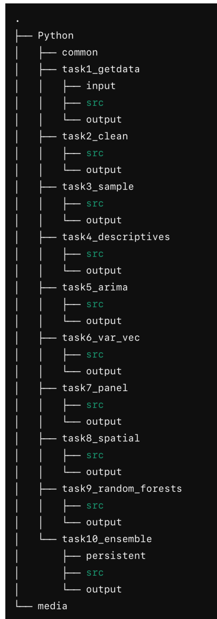
Figure 2: Toolbox overview.
